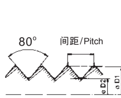
PG型螺纹
